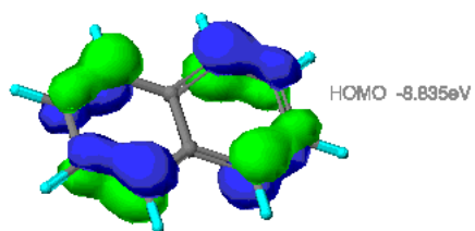
Naphthalene
