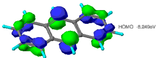
Anthracene
