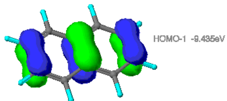
Anthracene
