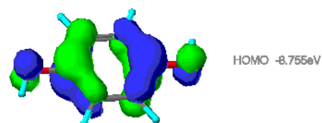
Hydroquinone
