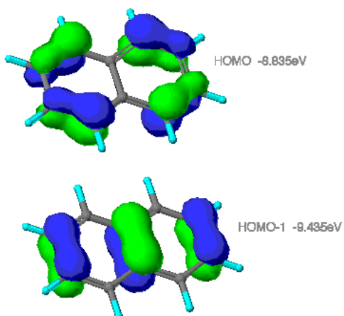
Naphthalene
