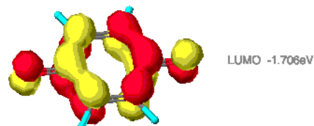
Hydroquinone
