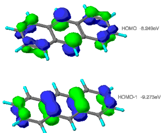
Anthracene
