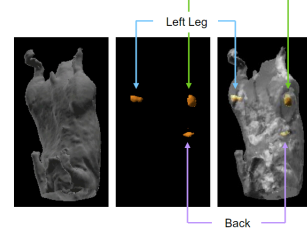
Fig. 7. Isosurface rendering of MRI and EPRI spin density map. From left to right, 3D MRI, final 3D EPRI spin density map generated from Eq. (2), and superposition of the two. For the EPRI reconstruction, the ROI was selected from the MRI.
