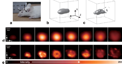
FIG. 7. EPR images of hydroxymethyl-PROXYL in the head of a subject mouse. a: Relation between the body of a mouse and Cartesian coordinates in laboratory space. b: Surface-rendered image obtained with a conventional method ( \sigma = 2.5 ). The field-of-view (FOV) of the image was 50 \times 50 mm. c: Surface-rendered high-resolution image obtained from the burned image in (b). d: Axial-slice images generated from the burned 3D image in (b). e: Axial-slice images of the 3D high-resolution image in (c). In (d) and (e), the FOV of the slice images was 25 mm. Background noise of \sim 10\% of the maximum signal intensity in the data set was suppressed in the slice images. Iteration was terminated at n = 20 with a threshold \sigma of 5 \times 10^{-6} . This iterative calculation took 245 s. The acquisition time for 3D projection data from a subject mouse was 60 s. The linewidth \Delta H_{1/2} of the zero-derivative spectrum was 0.445 mT for hydroxymethyl-PROXYL in the head of the mouse.
