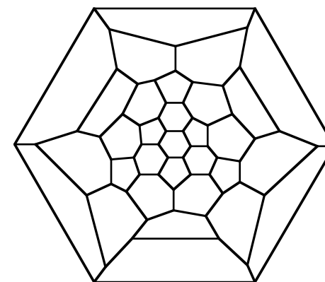
C60 Schlegel diagram
